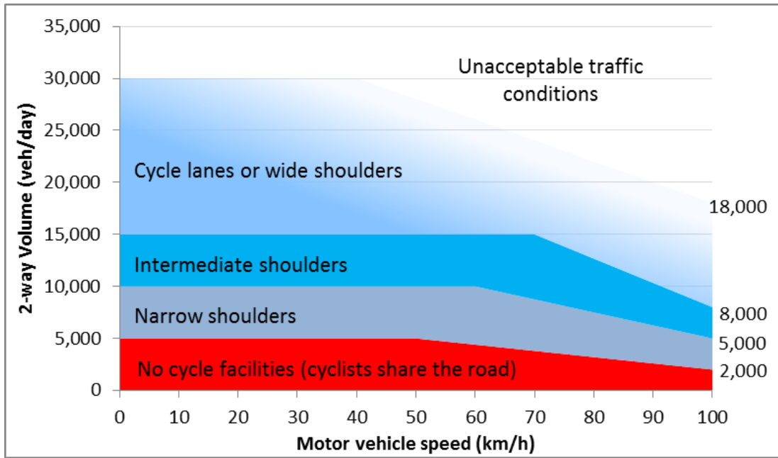
Figure 47: Trail type for Grade 5 on-road trails
