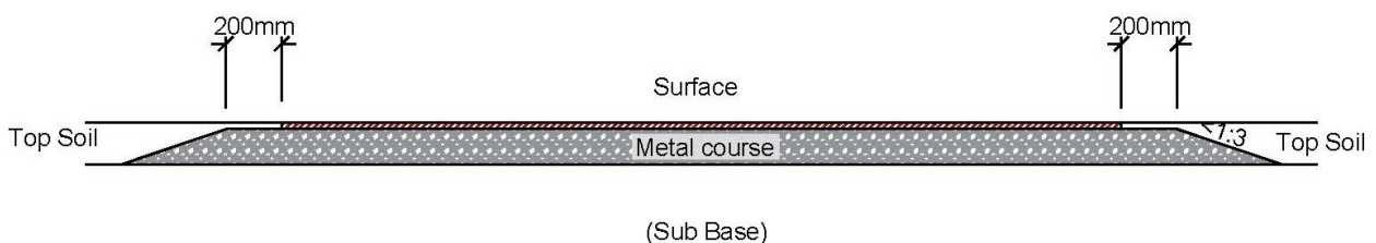
Figure 32: Cross section for chipseal or AC path without timber edging battens
